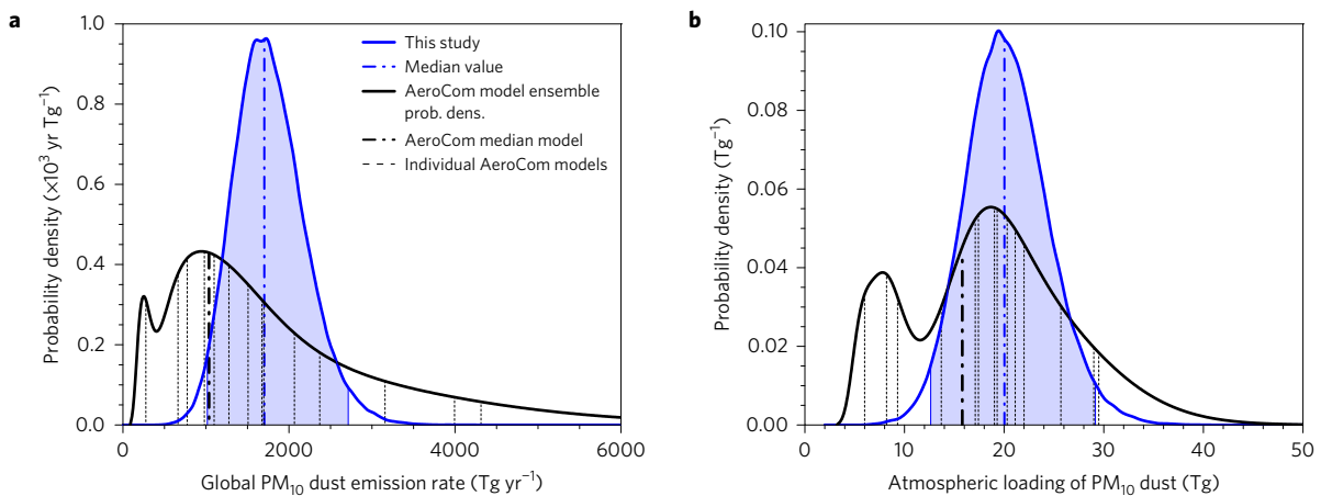
Figure 3 | Global emission rate and atmospheric loading of desert dust aerosols. a,b , Probability densities of the global dust emission rate ( a ) and atmospheric dust loading ( b ) (blue lines with shaded CI) indicate that some global models in the AeroCom ensemble 6 underestimate dust emission and loading.
